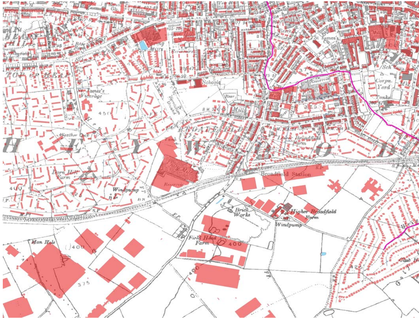
Figure 2 Land use change (infill) in the Wrigley Brook catchment Heywood, 1968 (black) to 2007 (red)
